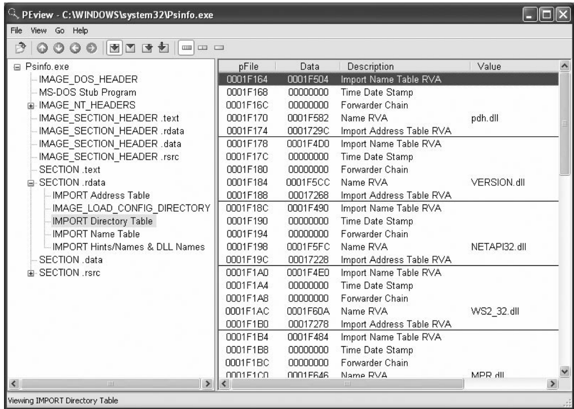
Figure 1.1 Identifying Required Libraries for psinfo with PEView
