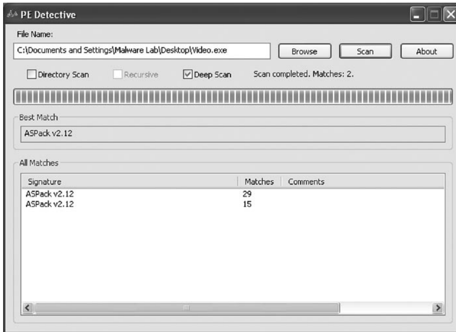
Figure 7.49 Examining Video.exe with PE Detectives
