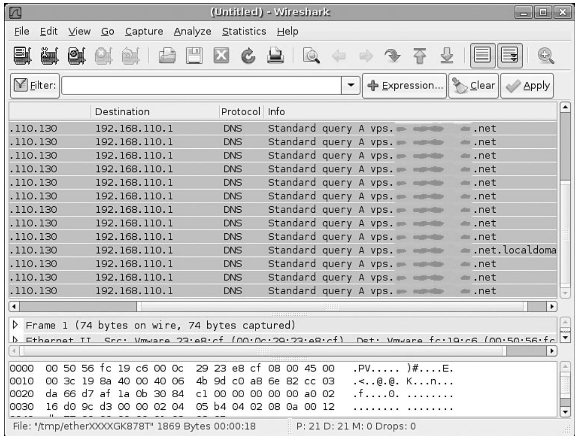
Figure 10.11 The Suspect Program Requesting to Resolve a Domain Name
