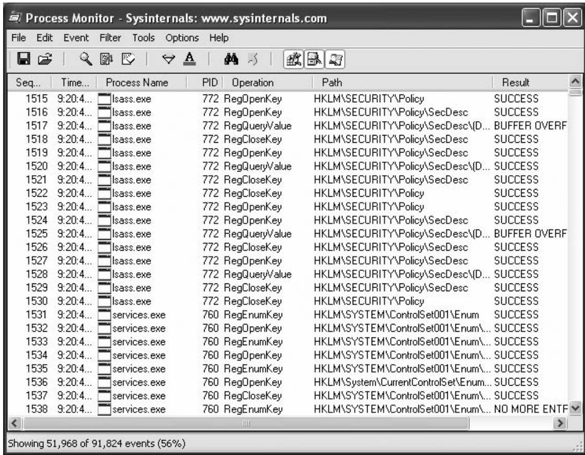
Figure 1.4 Process Monitor Displaying System Activity
