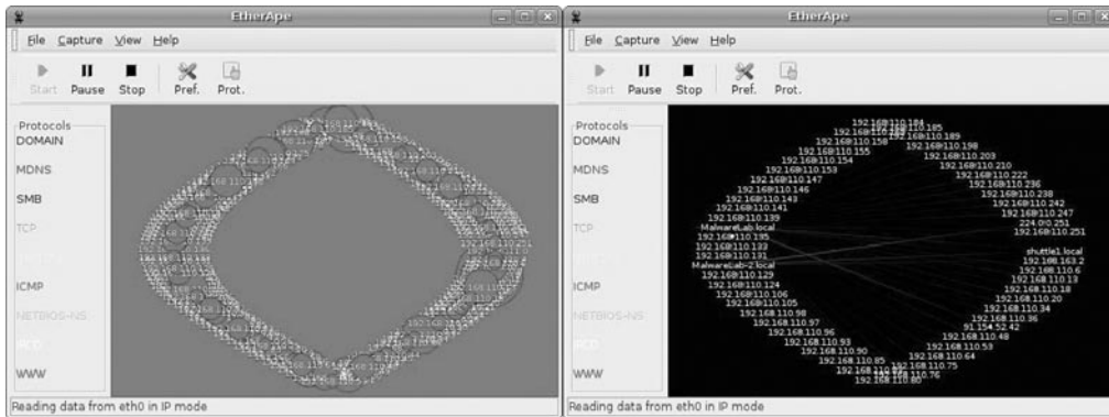
Figure 10.44 UDP Attack Manifesting in Etherape Traffic Visual
