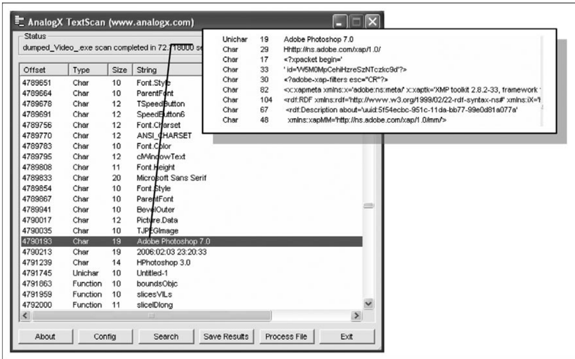
Figure 9.49 Discovering References to Adobe Photoshop in Strings
