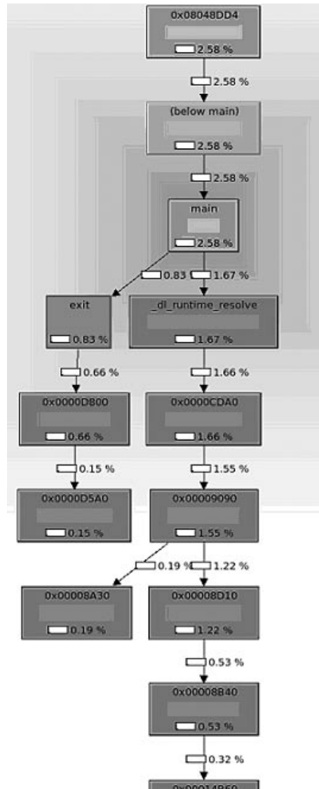
Figure 10.74 Callgrind Graph Created Using KCacheGrind
