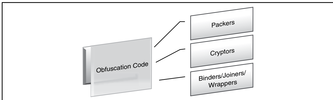
Figure 7.45 Obfuscating Code
