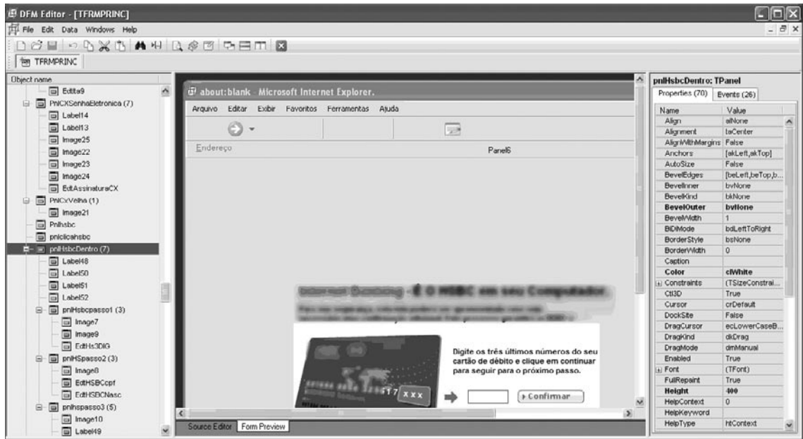
Figure 9.72 DFM Editor
