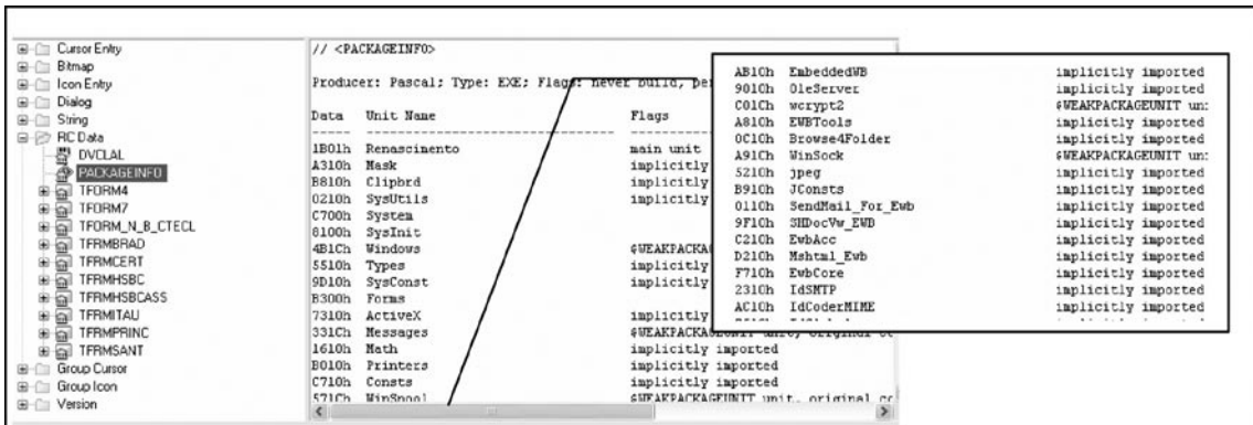
Figure 9.59 PACKAGEINFO
