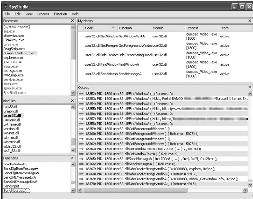
Figure 9.83 SpyStudio
