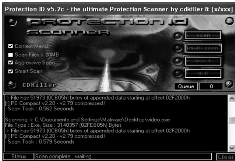
Figure 7.55 Protection ID
