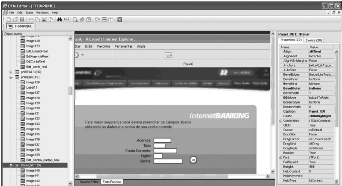
Figure 9.71 DFM Editor
