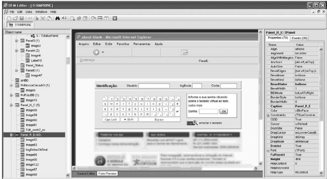
Figure 9.68 DFM Editor
