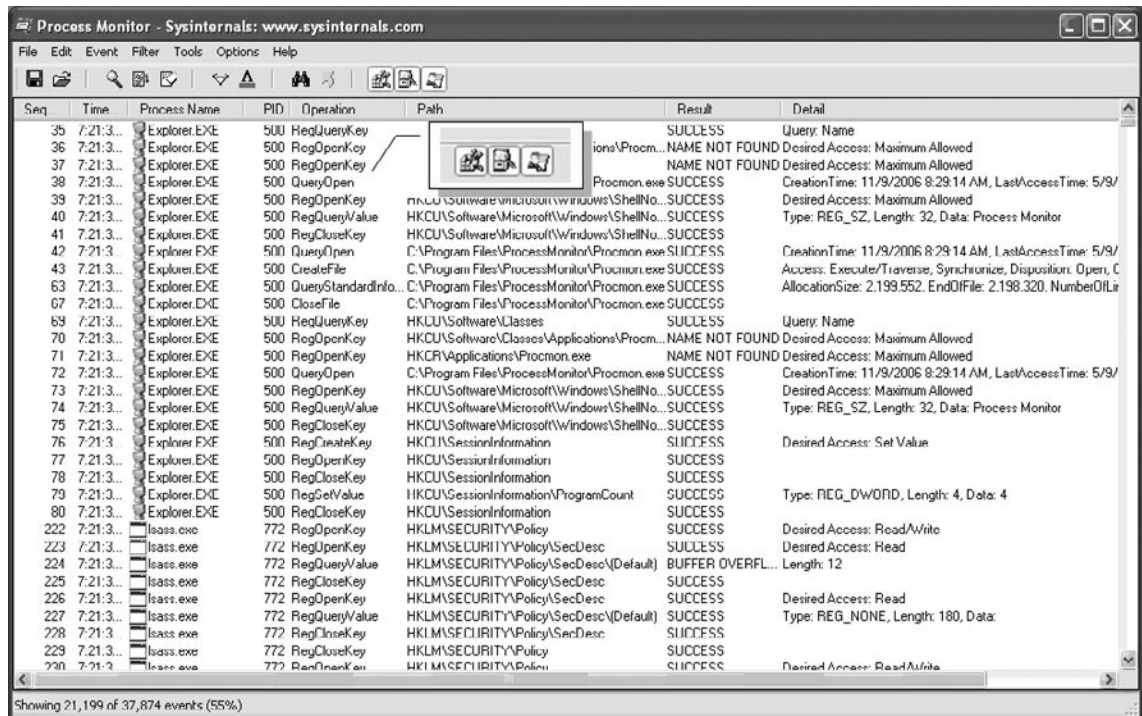
Figure 9.9 Process Monitor
