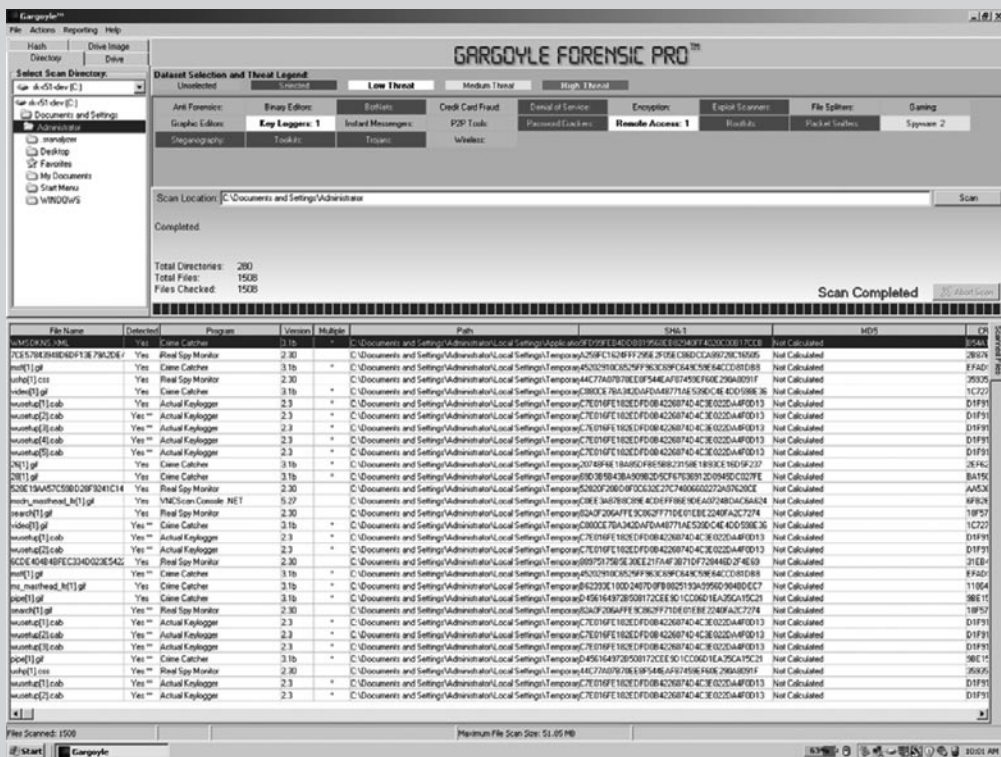
Figure 4.7 Gargoyle Example
