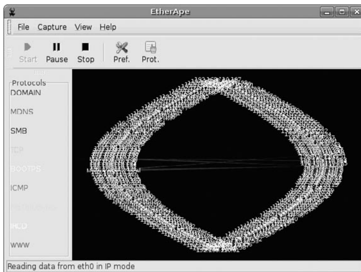
Figure 10.46 PAN Attack Manifesting in Etherape Traffic Visual
