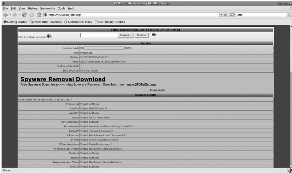
Figure 8.31 Jotti Online Malware Scan Results After Scanning Our Suspect File, sysfile
