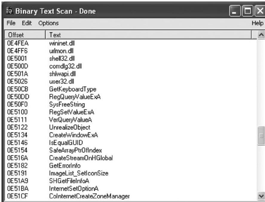
Figure 7.32 Identifying Function Calls and DLLs Using Binary Text Scan
