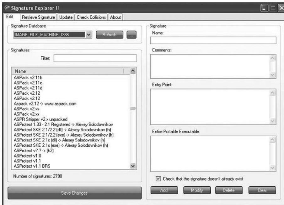
Figure 7.50 PE Detectives Signature Explorer
