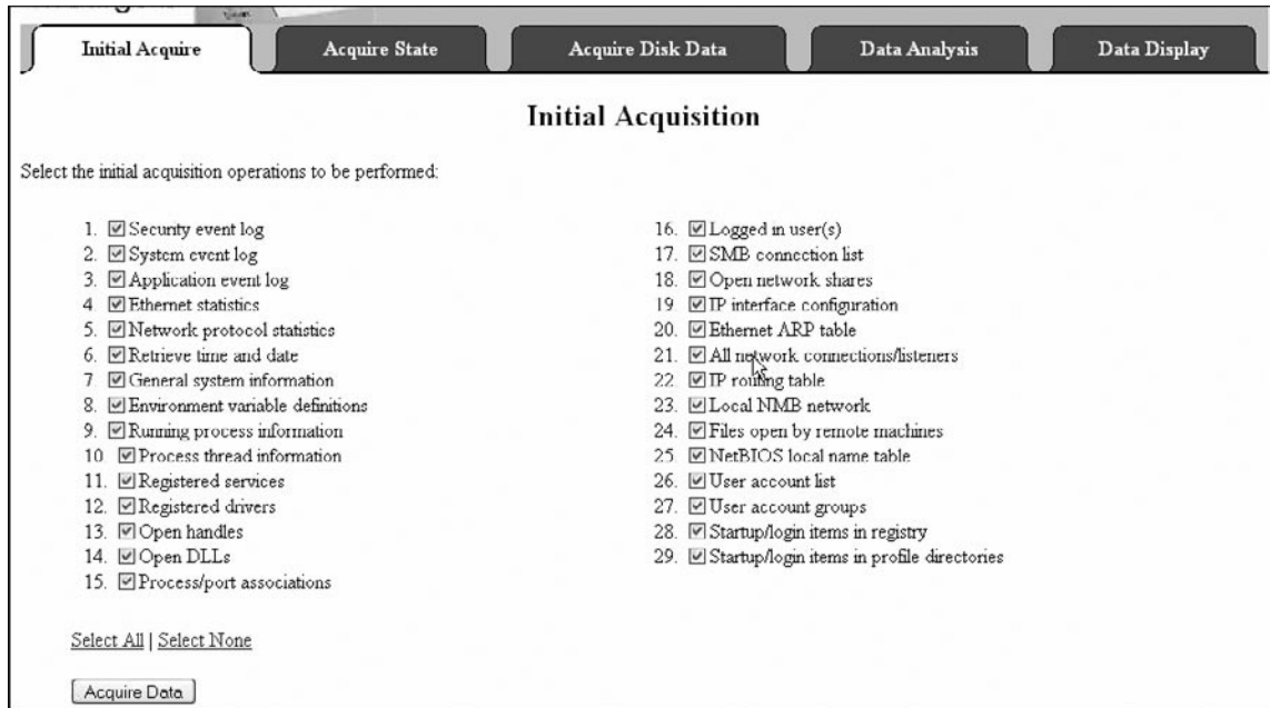
Figure 1.67 LiveWire
