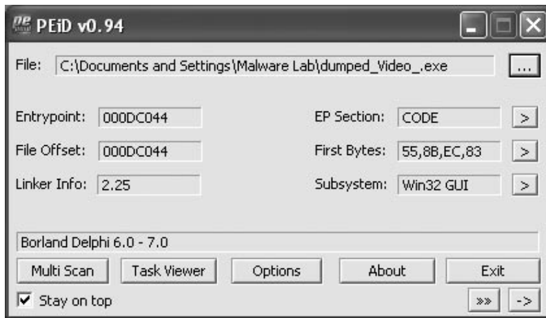
Figure 9.45 PEiD
