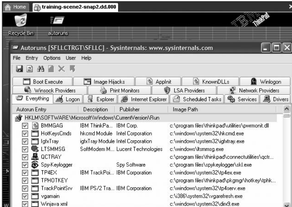
Figure 1.55 SysInternals Autoruns Tool for Detecting Autostart Locations, Running on a Forensic Duplicate of a Windows XP System Booted in a Virtualized Environment (VMWare) Prepared using LiveView
